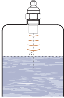
Fig. 1: Recommended installation
